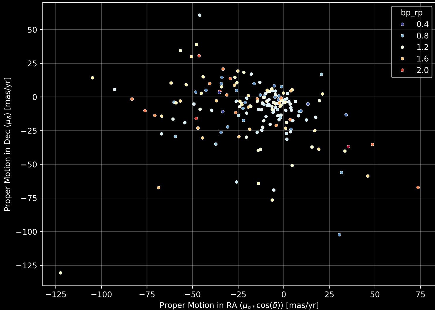
APOGEE DR17 Field: [277+76] Proper Motion Diagram (n= 184)
