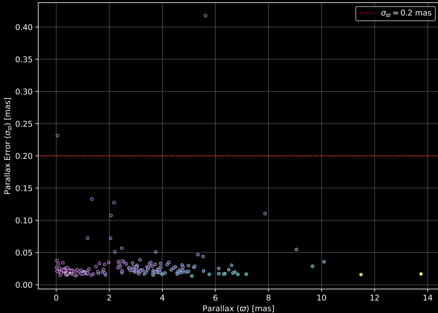
APOGEE DR17 Field: [277+76] Parallax Quality (n= 184)
