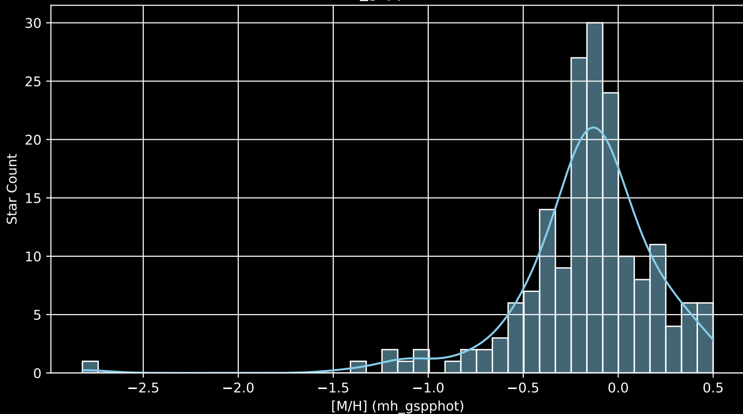
APOGEE DR17 Field: [277+76 [M/H] (mh_gspphot) (n= 177)
