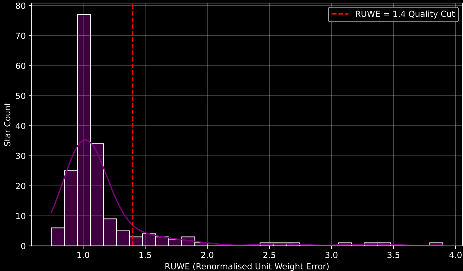
GAPOGEE DR17 Field [277+76] RUWE Distribution (n= 179)
