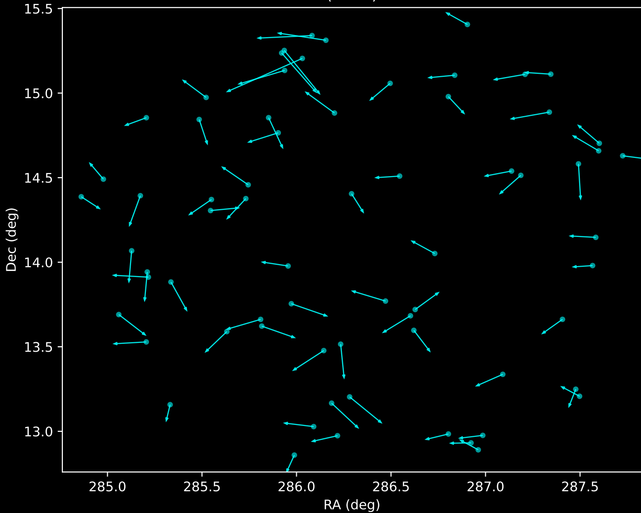
APOGEE DR17 Noise Stream Proper Motion Vectors (n=68)
