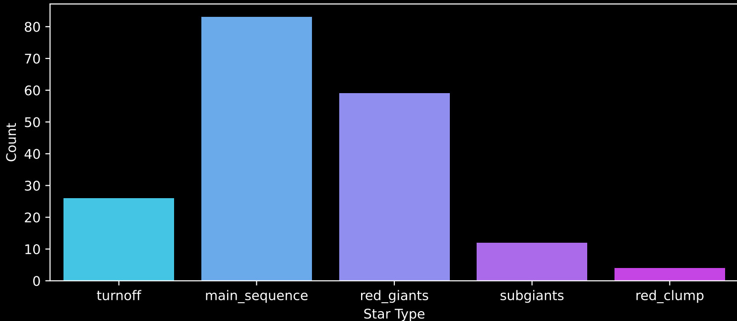
APOGEE DR17 Field: [277+76] Count plot of Star Type
